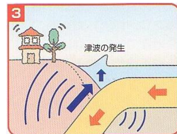
When the stress comes to its limit, the continental plate suddenly springs up. That is an earthquake. It may cause tsunami.
