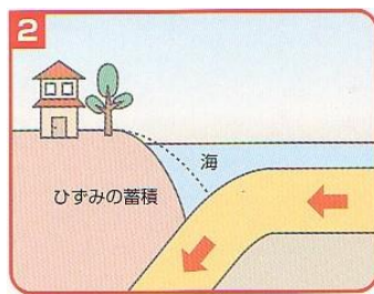
The head of the continental plate is strained by the movement. The elastic strain energy around the plate boundary is increasing.
